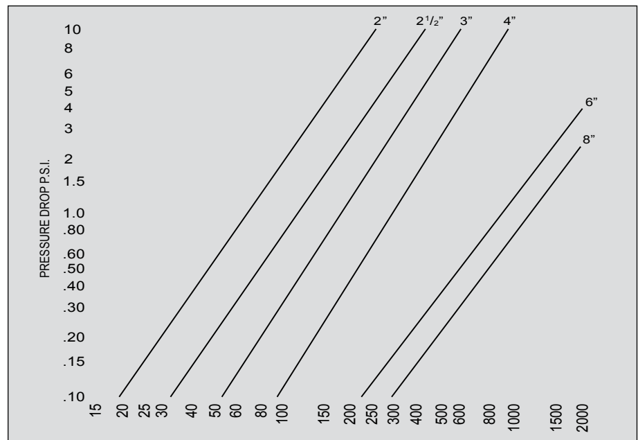
FLOW RATE (WATER) G.P.M.
